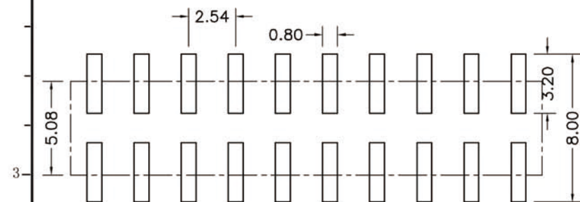
P. C. B LAYOUT
