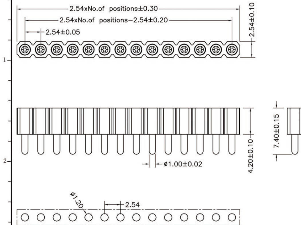
P. C. B LAYOUT
