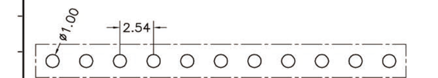
P. C. B LAYOUT
