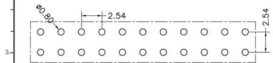
P. C. B LAYOUT
