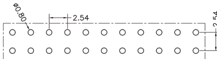
P. C. B LAYOUT
