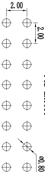
PCB LAYOUT
