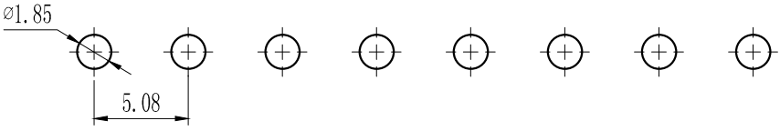
PCB LAYOUT
