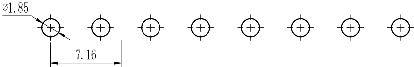
PCB LAYOUT
